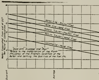
Evaporation from and at 212° per lb. of combustible
